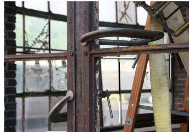
[20 a-d] The original steel windows in this industrial building were successfully repaired as part of the rehabilitation project (left).
